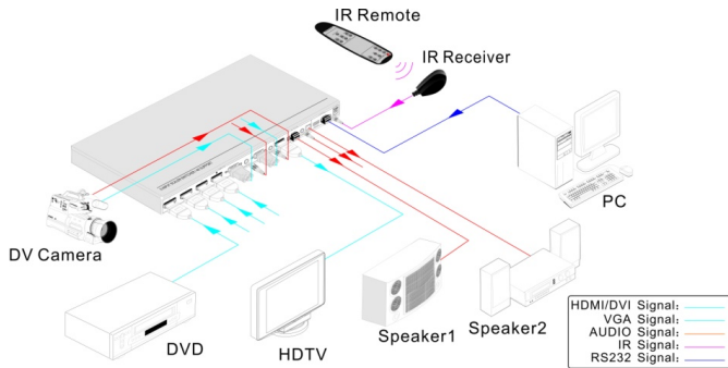
Figure 3- 1 Connection Diagram
