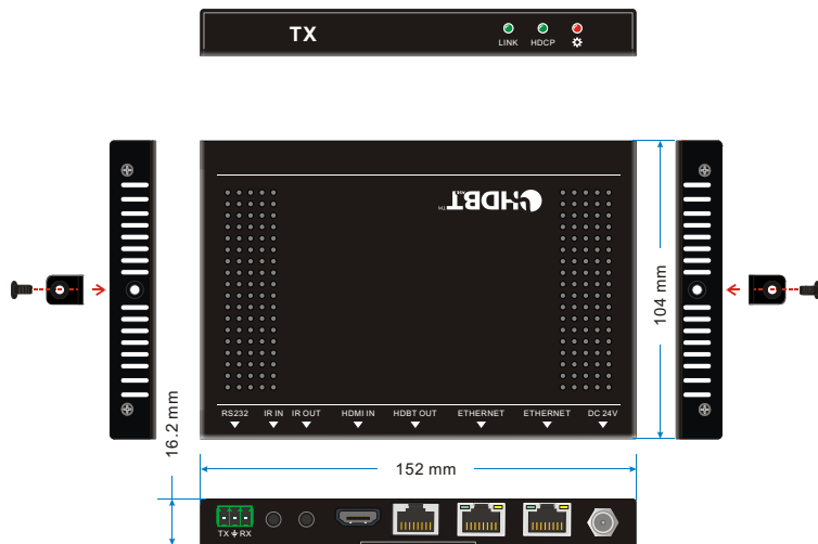
5-1 TPUH422T Transmitter
